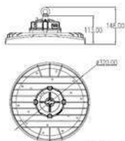
200W/240W
