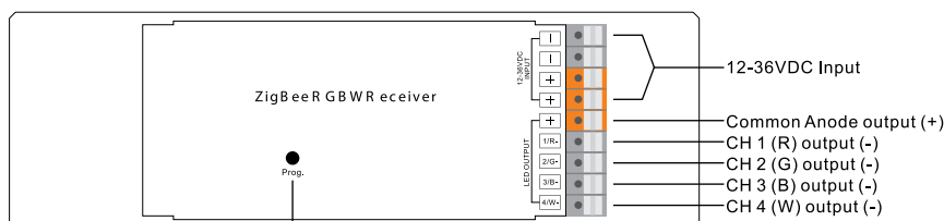
LC-ZG-9101FA-RGBW
