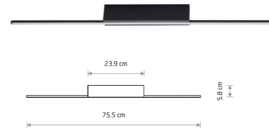
GIAVELLOTTO LED S painted steel, painted aluminum, plastic PC
