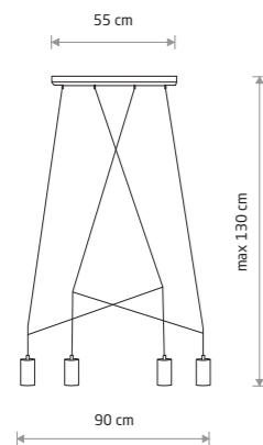
IMBRIA painted steel, braided cable
