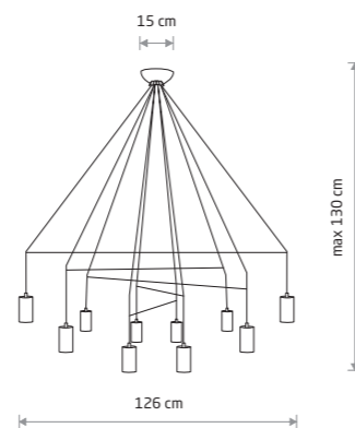
IMBRIA painted steel, braided cable
