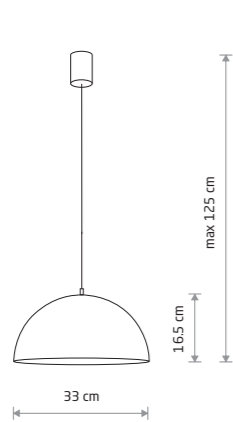
HEMISPHERE RUST S
