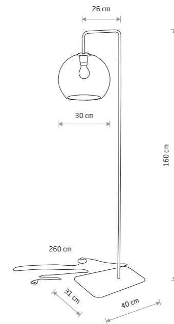
MONACO painted steel, glass
