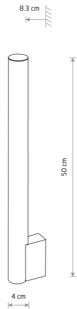
ICE TUBE LED M plastic PC, chrome plated steel
