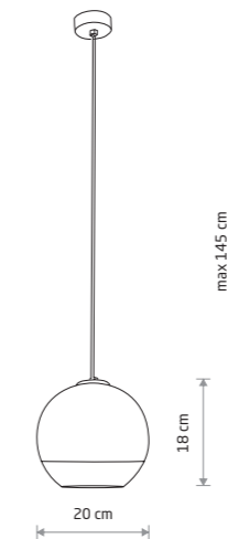
GLOBE PLUS S metallized glass, painted steel
