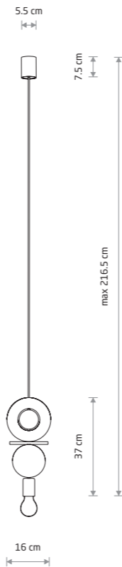
DROPS WOOD E plywood, painted steel
