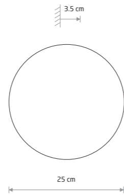
RING WOOD LED M
