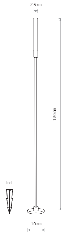
ZOLA LED painted aluminum, plastic PC ■ 11546 ●
