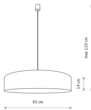
TURDA fabric, plastic, painted steel
