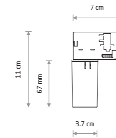
CAMELEON ADAPTER CTLS plastic
