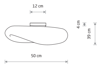
HAVANA S bamboo, painted steel, plastic ABS
