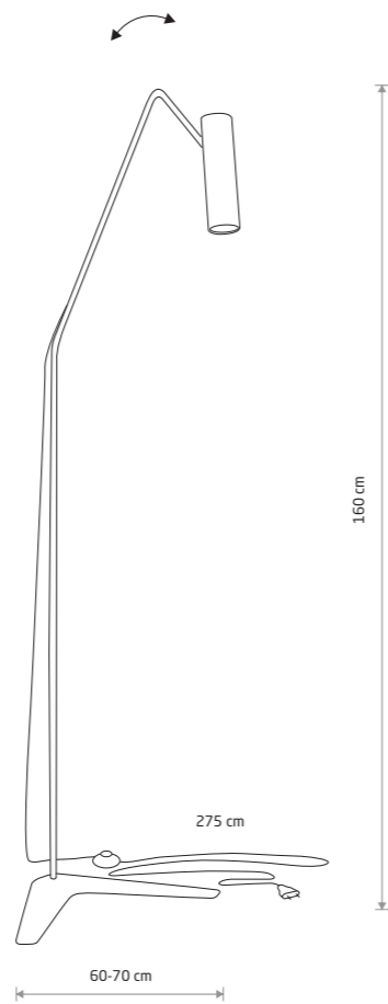
EYE SUPER painted steel
