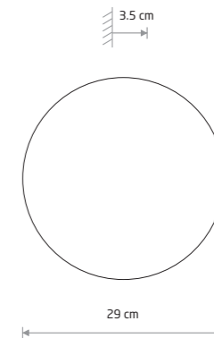
RING MIRROR LED M glass, painted steel
