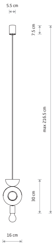
DROPS WOOD F plywood, painted steel
