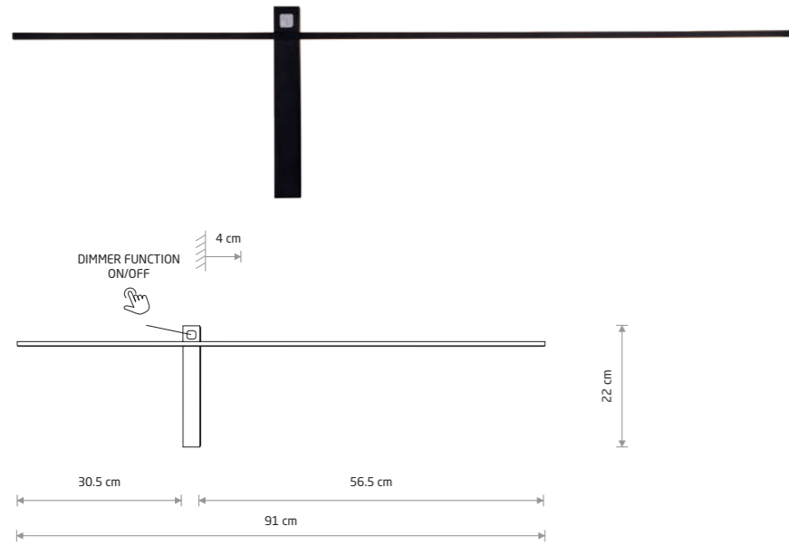
IMPULSE LED M 8116
