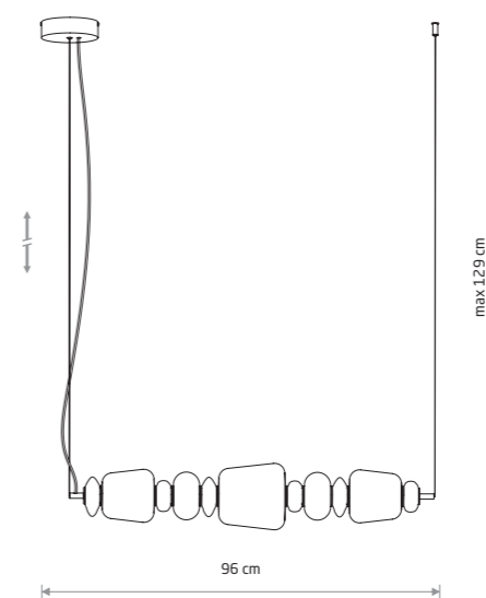
CERAMIC LED glass, ceramic housing
