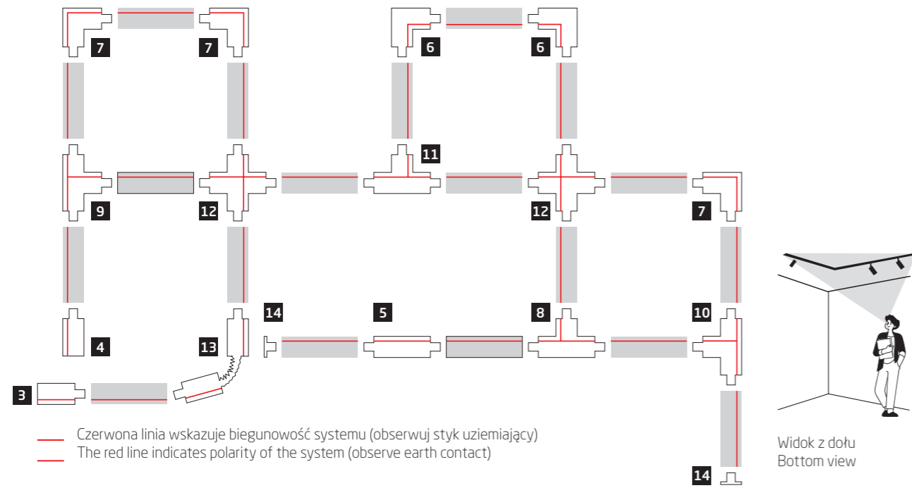
3 CTLS RECESSED POWER END CAP, RIGHT (PE-R) plastic, copper
