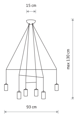
IMBRIA painted steel, braided cable
