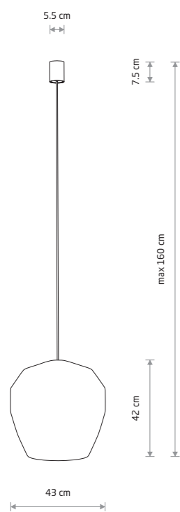
HAITI S bamboo, painted steel
