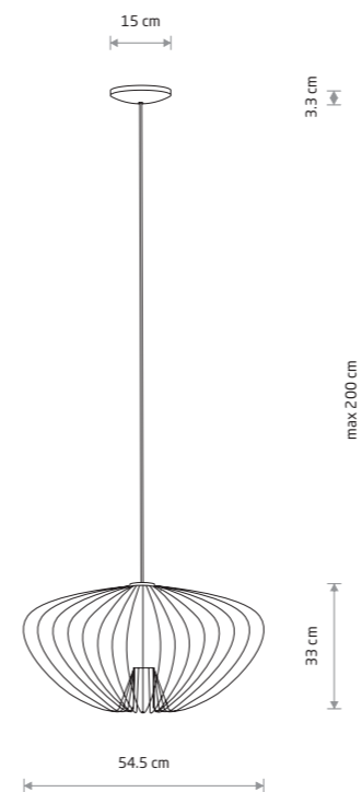
PUMPKIN M
