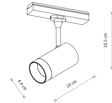
UT-LVM SPOT LED 9W
