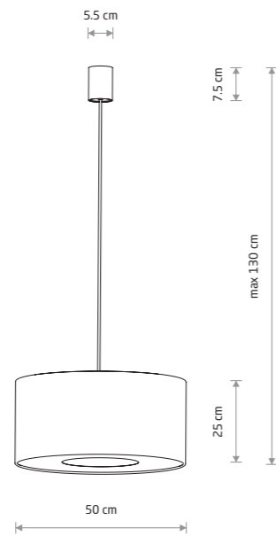
CEDRO M fabric, painted steel, plastic
