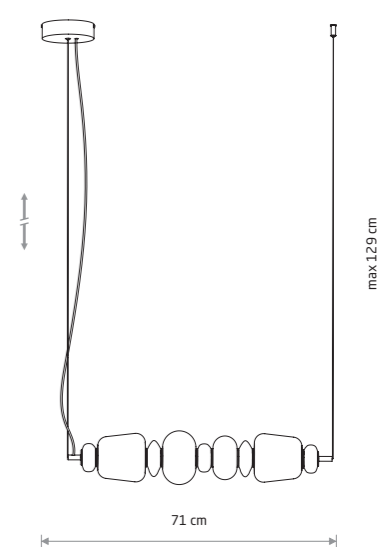
CERAMIC LED glass, ceramic housing
