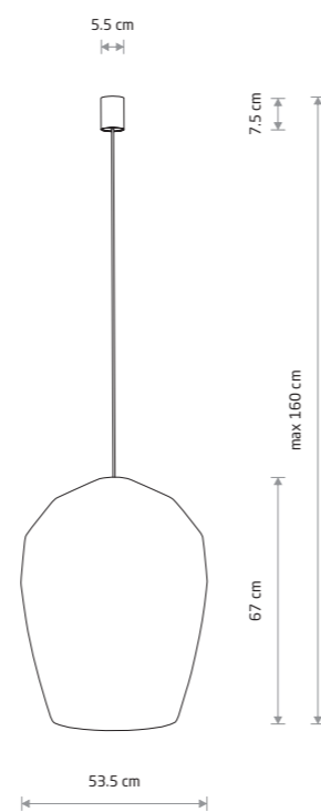
HAITI L bamboo, painted steel
