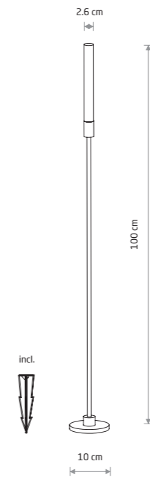
ZOLA LED painted aluminum, plastic PC ■ 11545 ●
