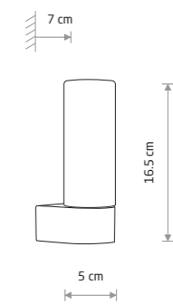
NATALIE aluminum, glass
