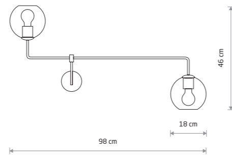
MONACO glass, painted steel
