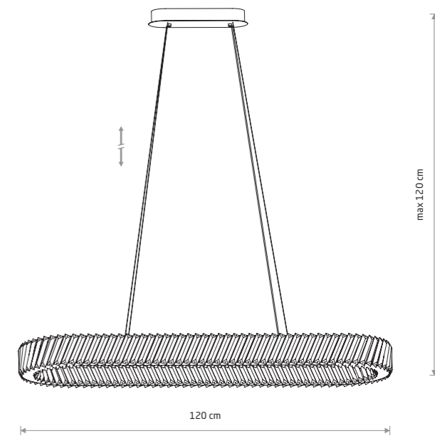
LUXORA LED
