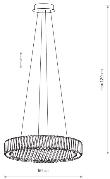
LUXORA LED
