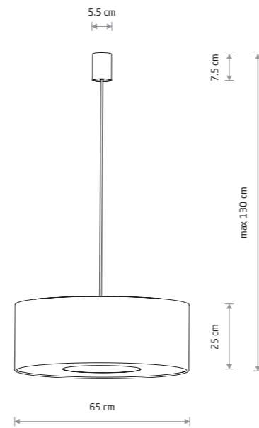
CEDRO L fabric, painted steel, plastic
