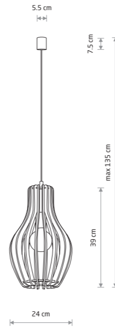
IKA A plywood, painted steel 4171 1x E27, max 25W only LED
