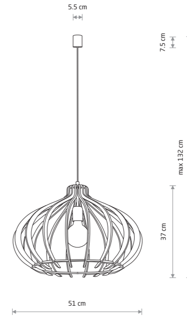
IKA D plywood, painted steel 4174 1x E27, max 25W only LED
