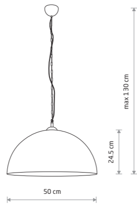
HEMISPHERE RUST L
