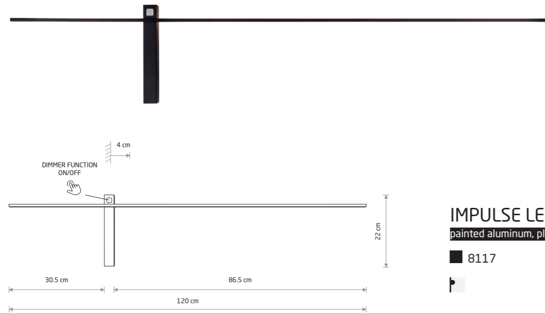
IMPULSE LED L 8117
