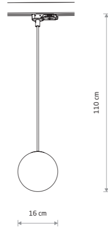
CTLS SNOWBALL plastic PC, glass, painted steel
