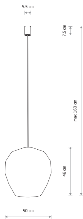
HAITI M bamboo, painted steel
