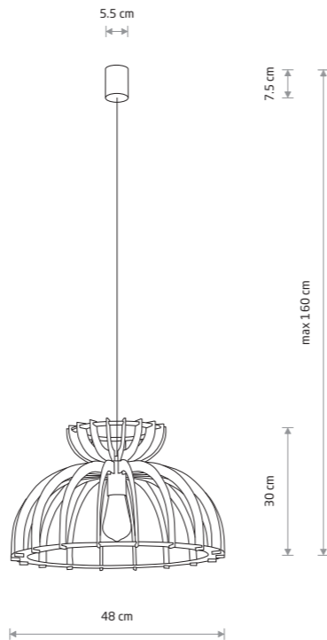
KYMI C plywood, painted steel, braided cable 10572 ■ 10575 1x E27, max 25W only LED
