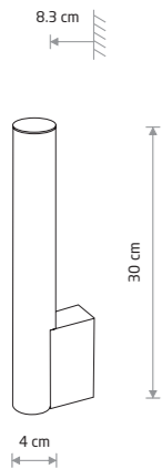
ICE TUBE LED S plastic PC, chrome plated steel
