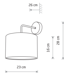
ALICE fabric, painted steel
