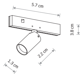
NANO - LVM SPOT LED 1W
