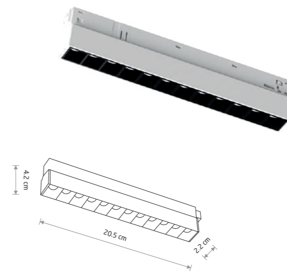
LVM FOCUS LED 9W 11632
