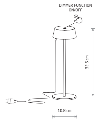
AMY LED 11534
