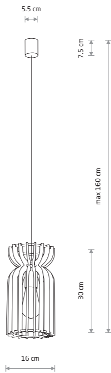
KYMI B plywood, painted steel, braided cable 10571 ■ 10574 1x E27, max 25W only LED
