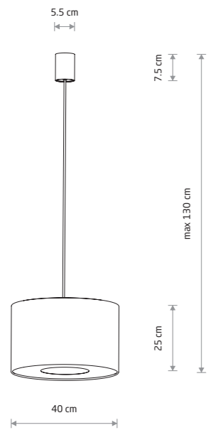
CEDRO S fabric, painted steel, plastic
