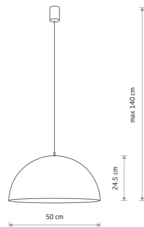
HEMISPHERE HIT L
